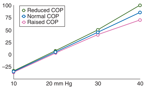
Fig 3 Autotransfusion. Transendothelial filtration rate J_v is proportional to the capillary pressure, or transendothelial pressure difference if interstitial pressure is not constant. Normal capillary pressure is nominally 20 mm Hg, and the scale for J_v is arbitrary, although studies show the rate of clearance from the intravascular space during rapid infusion of Ringer's acetate in humans can be as much as 100 ml min -1 . Raising the plasma COP slows filtration (pink line), while reducing plasma COP increases it (green line).
