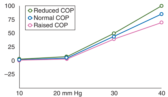
Fig 4 The no absorption rule. With less acute reduction in capillary pressure, the glycocalyx model preserves filtration at a very low rate without a phase of absorption, the no absorption rule. We call the inflection on the filtration curve the J point.
